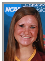
Malleri Hardison
