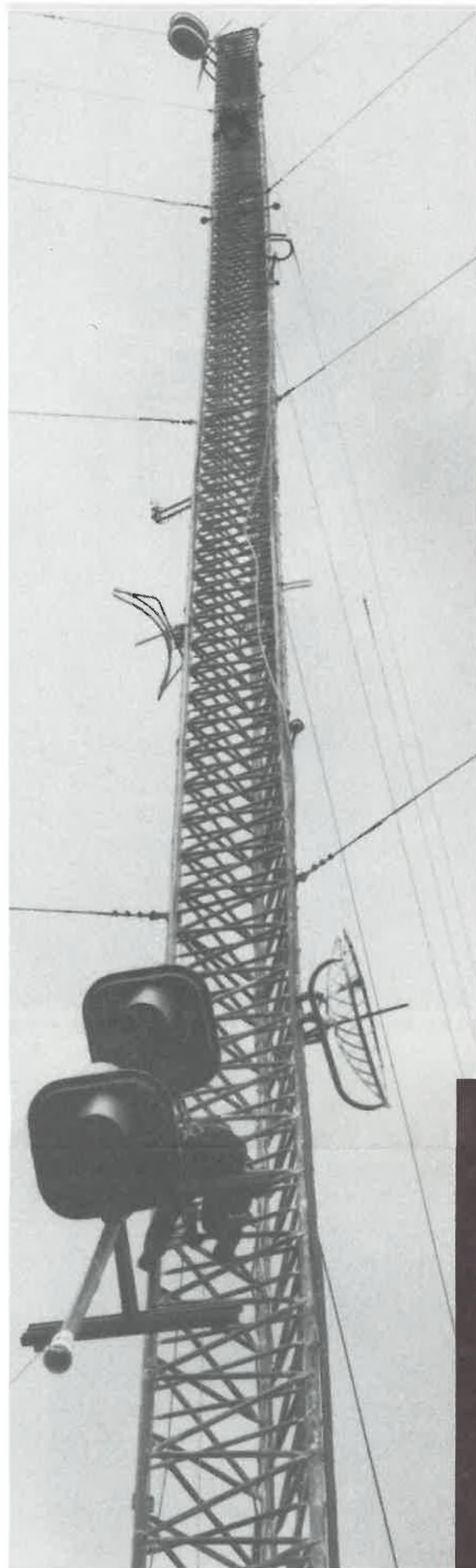
WCDR's new antenna is raised on the tower to make possible the power increase from 3,000 to 30,000 watts.
