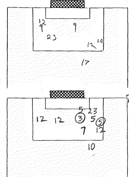
SHOT CHART
